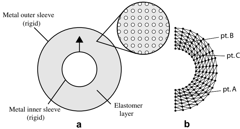
Fig. 16. Geometry of the elastomer bushing problem.
